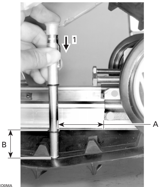
1. Belt tension tester
